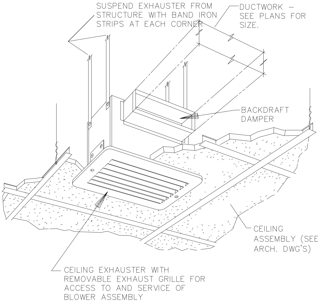
CEILING MOUNTED FAN DETAIL D 04 SCALE NTS
