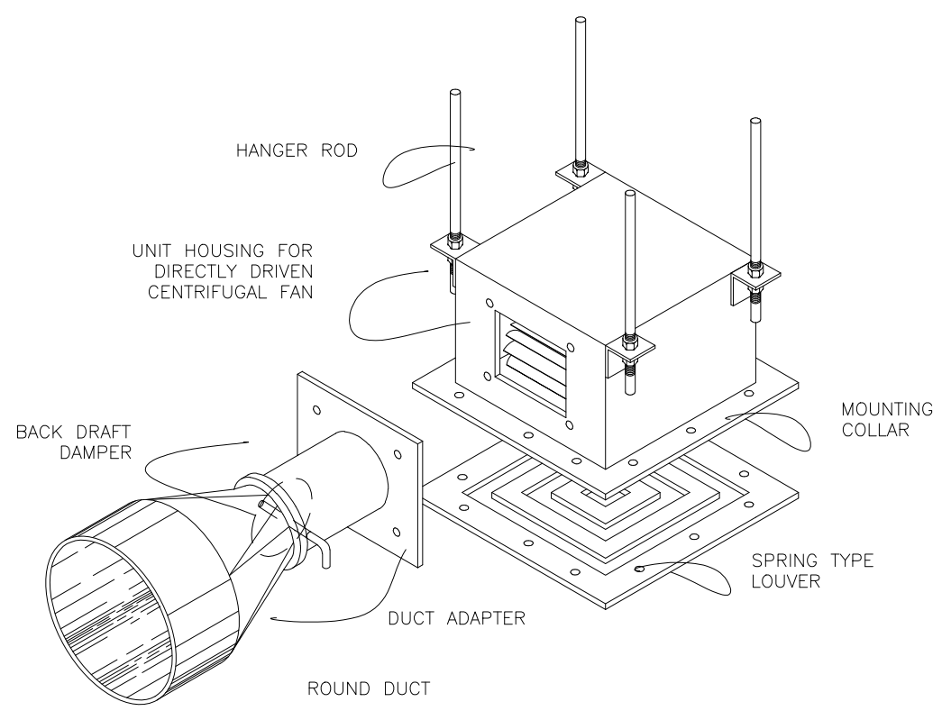
CEILING EXHAUST FAN DETAIL ( ROUND ) D 09 SCALE NTS
