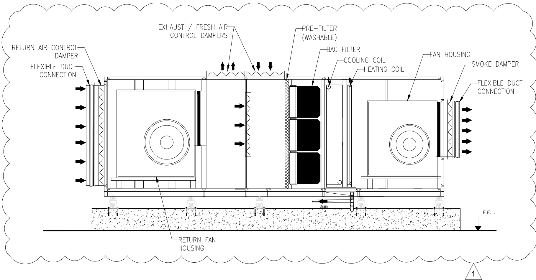
TYPICAL AHU INSTALLATION DETAILS D 05 SCALE NTS
