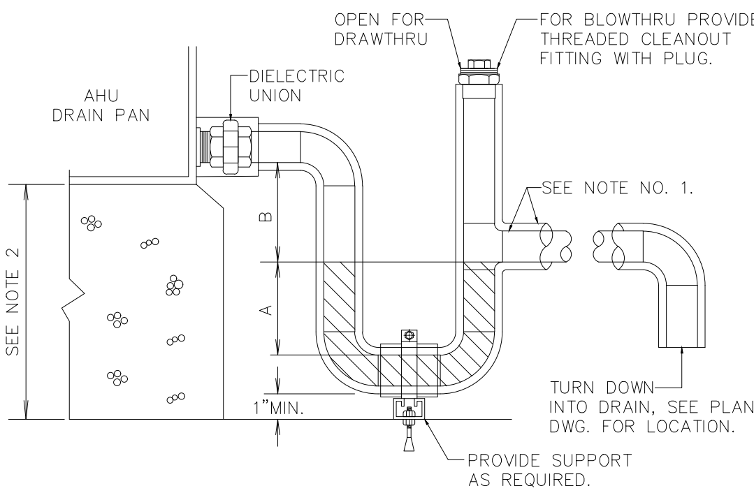
CONDENSATE DRAIN DETAIL D 07 SCALE NTS
