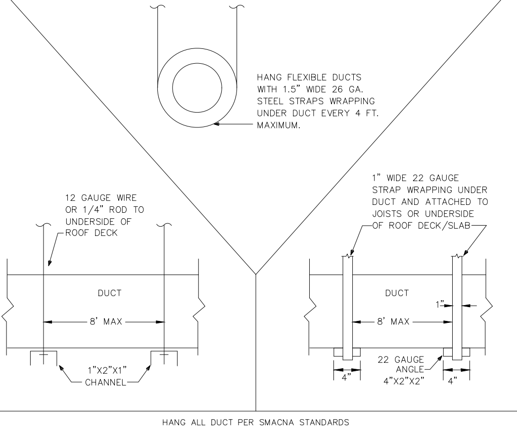
DUCT SUPPORT DETAIL D 11 SCALE NTS
