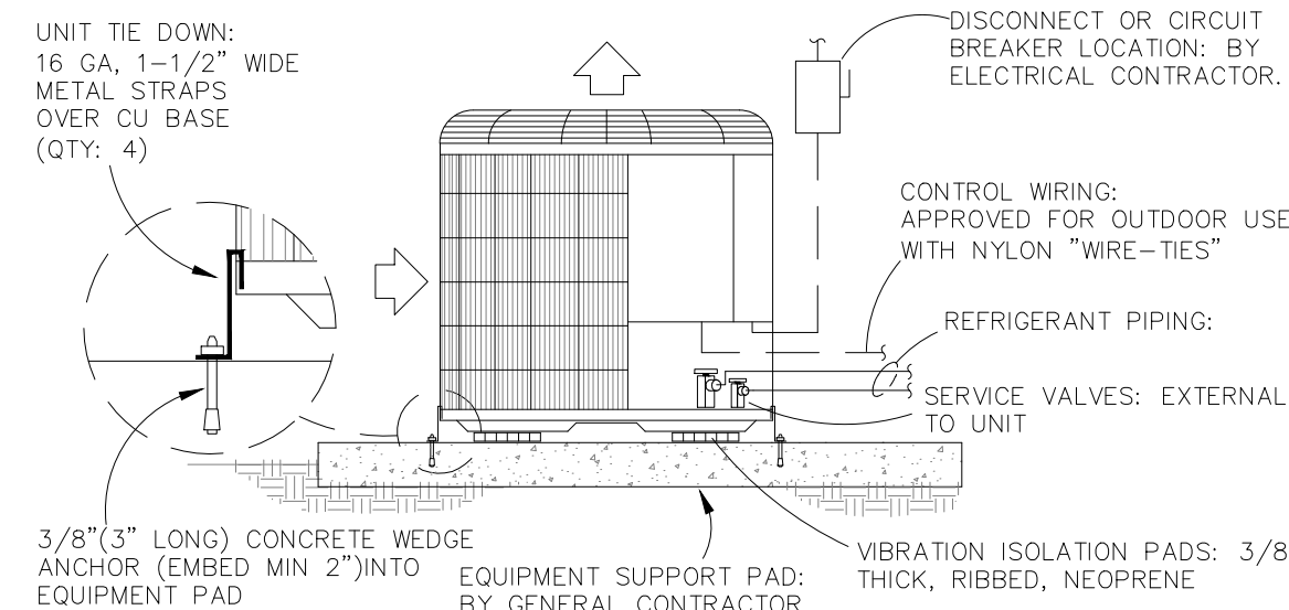
CONDENSER MOUNTING DETAIL D 10 SCALE NTS
