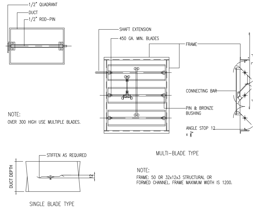
VOLUME DAMPER DETAIL D 08 SCALE NTS
