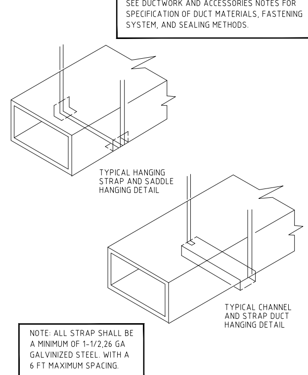
METHODS OF HANGING RIGID FIBERGLASS DUCT DETAIL D 12 SCALE NTS
