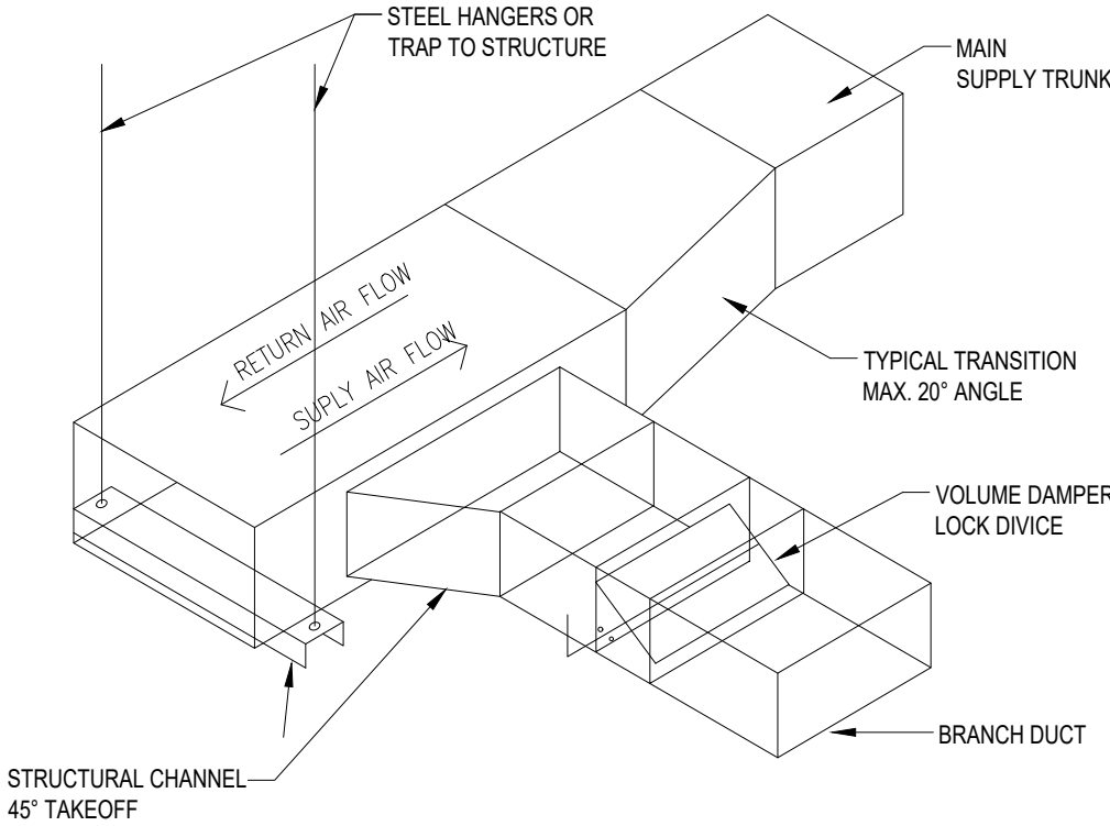
BRANCH DUCT TAKEOFF DETAIL D 06 SCALE NTS
