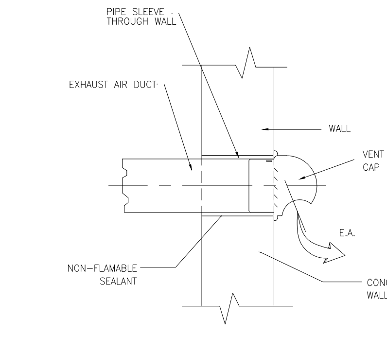
EXHAUST AIR VENT CAP DETAIL D 14 SCALE NTS
