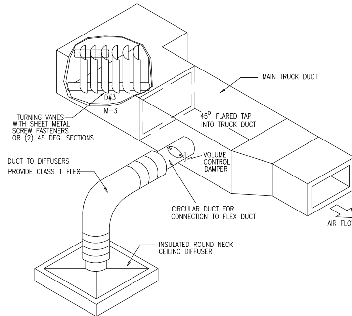
TURNING VANES DETAIL D 03 SCALE NTS
