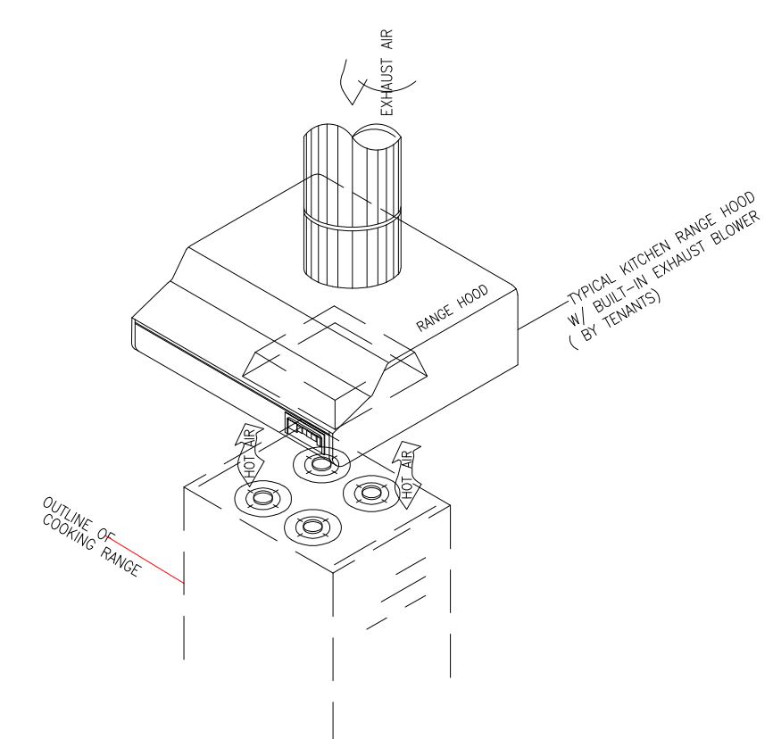
KITCHEN EXHAUST INSTALLATION DETAIL D 13 SCALE NTS
