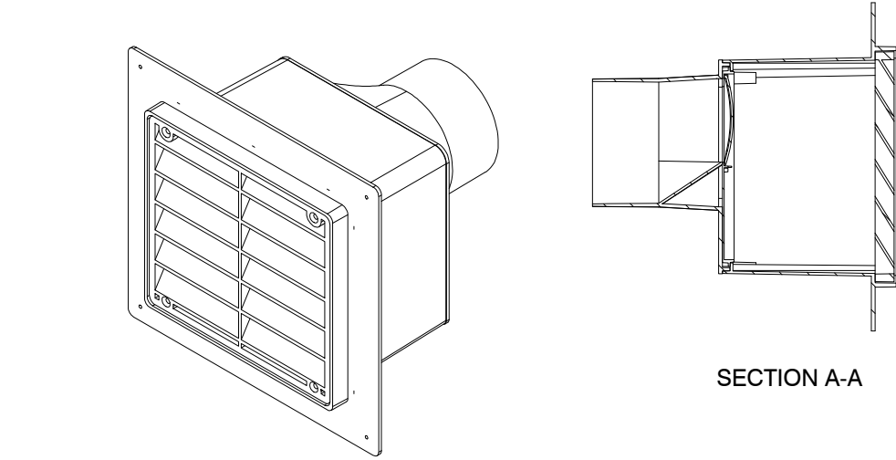
TYPICAL VENT LOUVER TERMINATION AT WEATHER D 02 SCALE NTS
